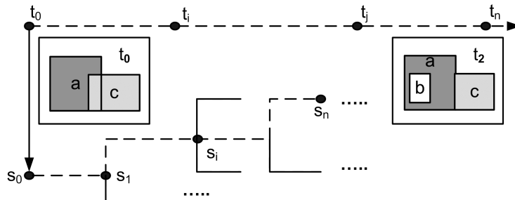
Figure 5. Abductive explanation.
